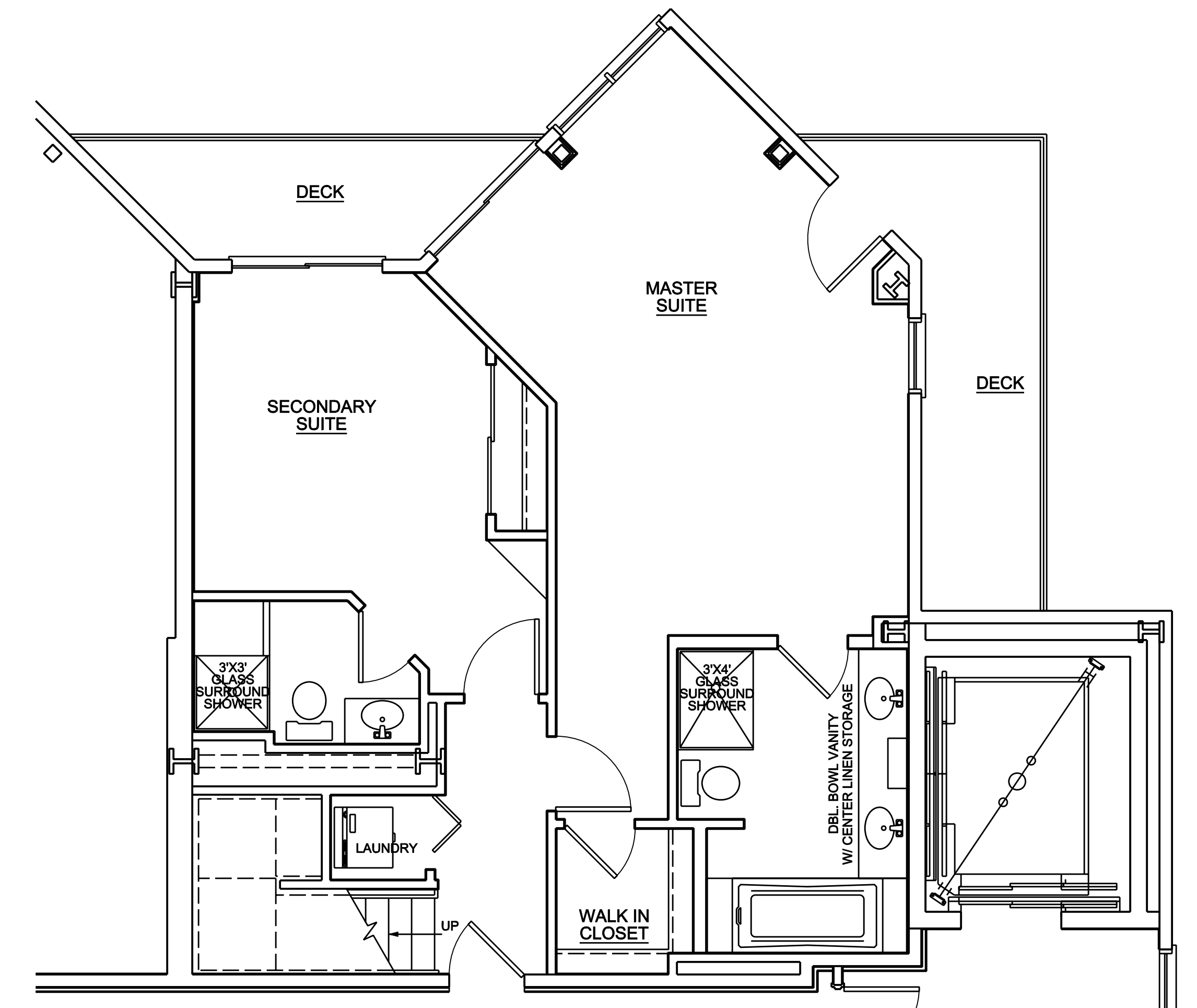
2 TOWNHOUSE E - LOWER LEVEL A7.3 SCALE: 1/4"=1'-0"
