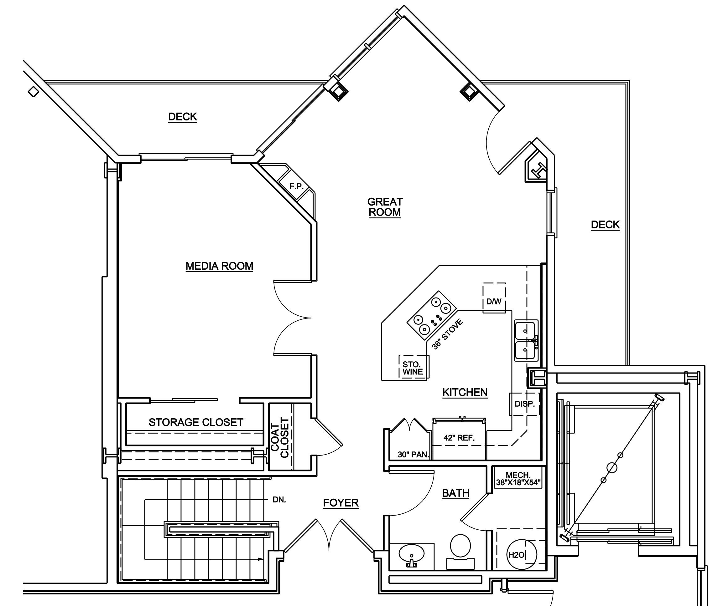
1 TOWNHOUSE E - UPPER LEVEL A7.3 SCALE: 1/4"=1'-0"
