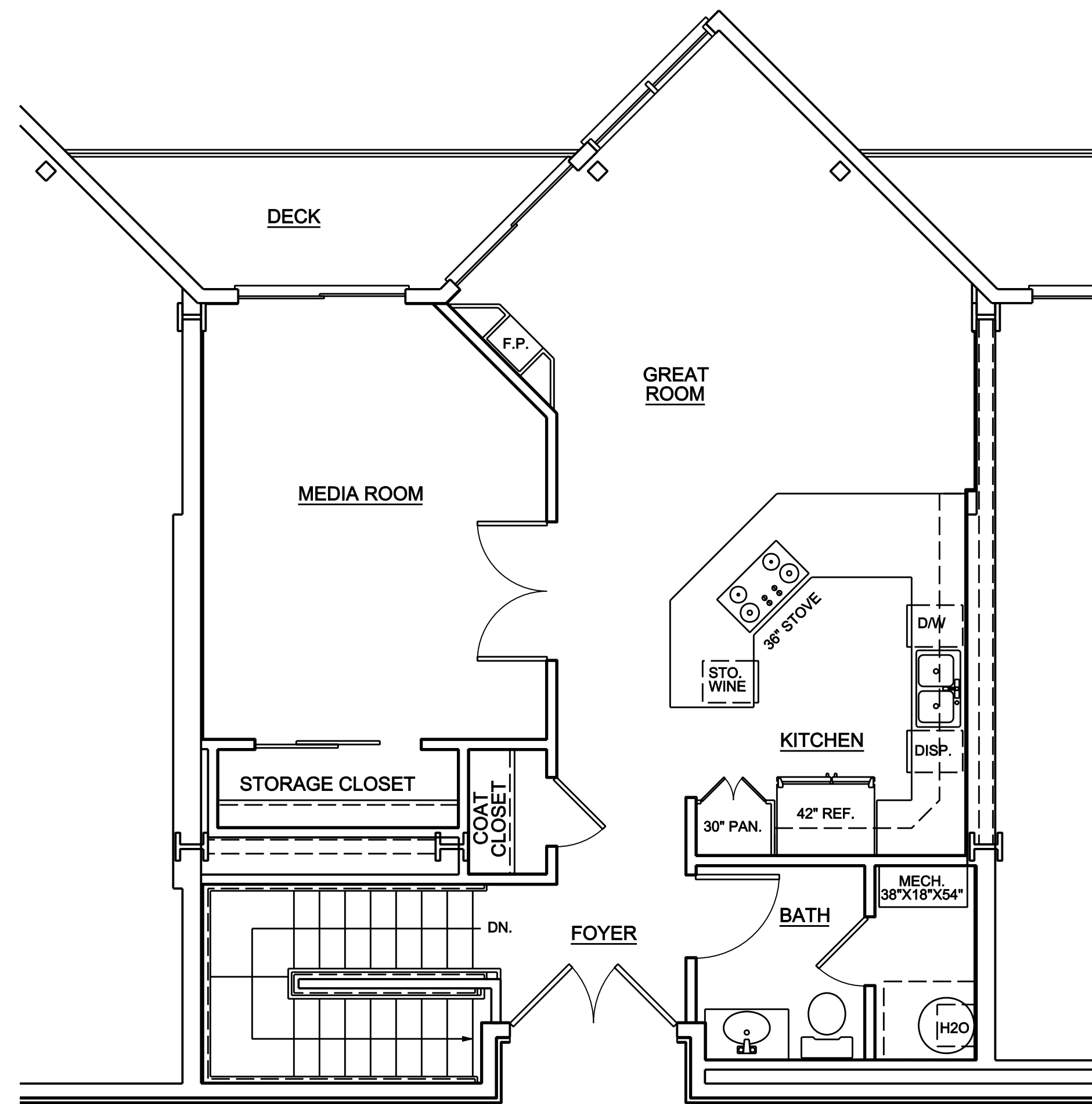
3 TOWNHOUSE F - UPPER LEVEL A7.3 SCALE: 1/4"=1'-0"
