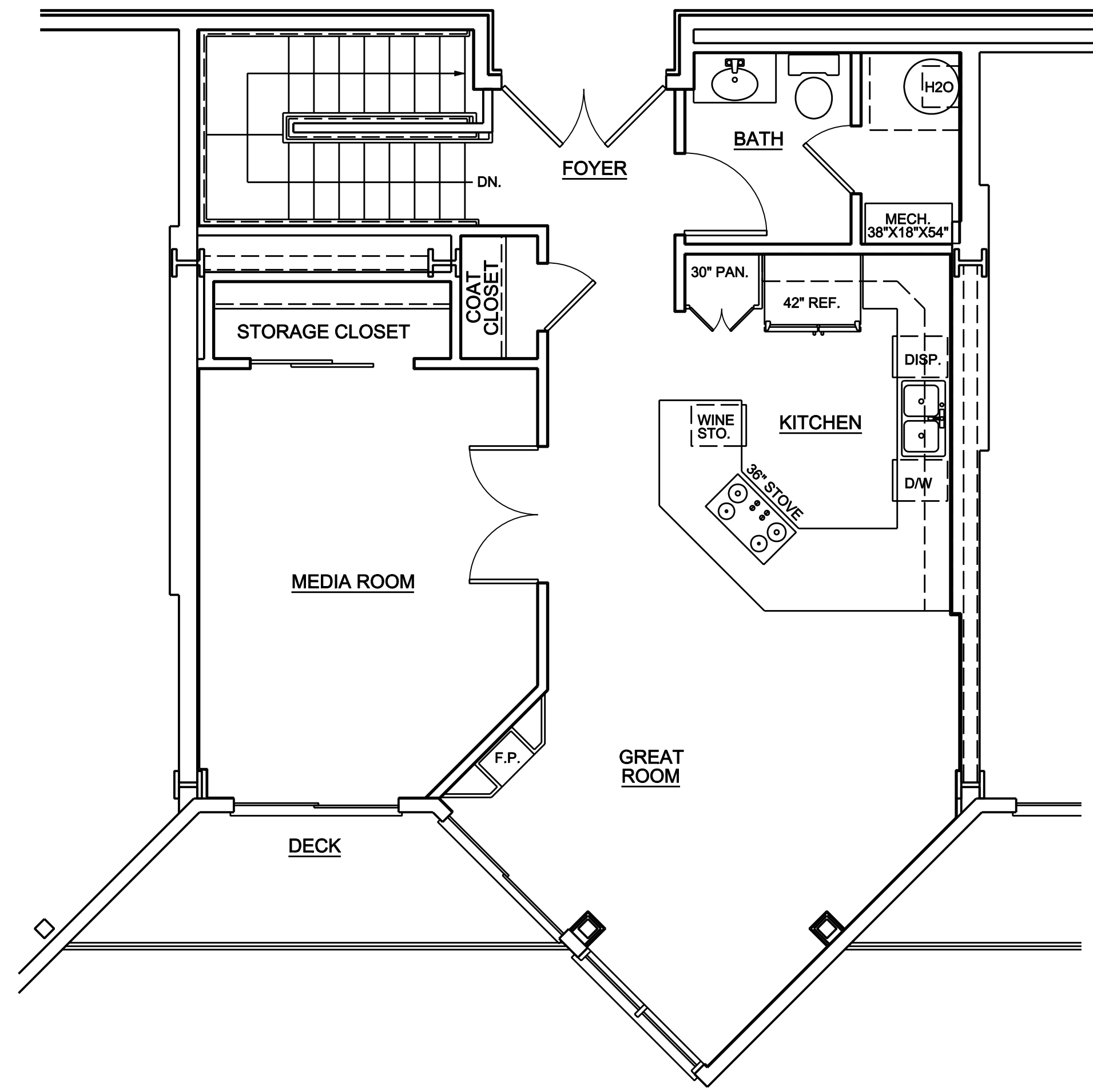
5 TOWNHOUSE G - UPPER LEVEL A7.3 SCALE: 1/4"=1'-0"
