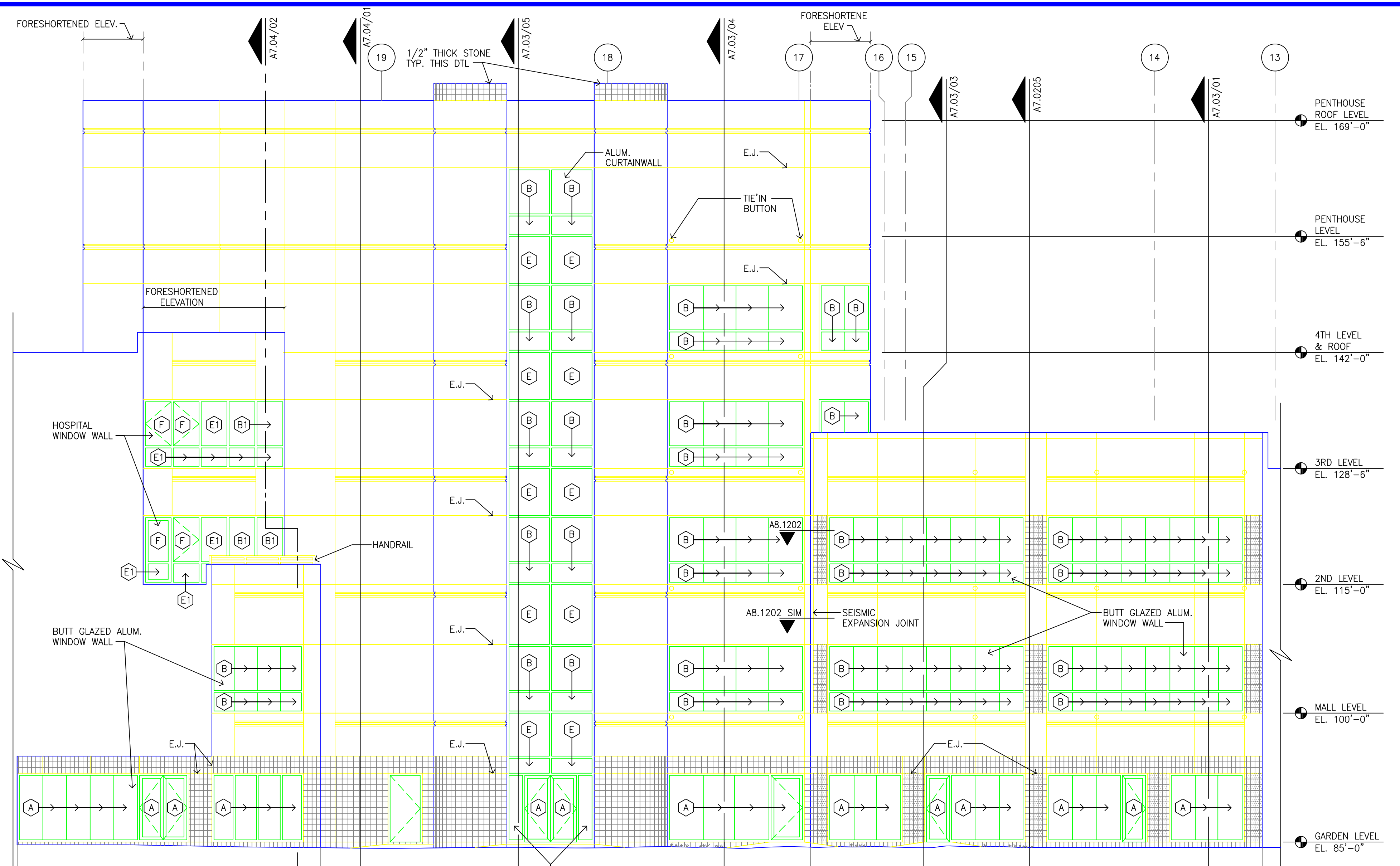
03 NORTH ELEVATION ELEVATOR TOWER
