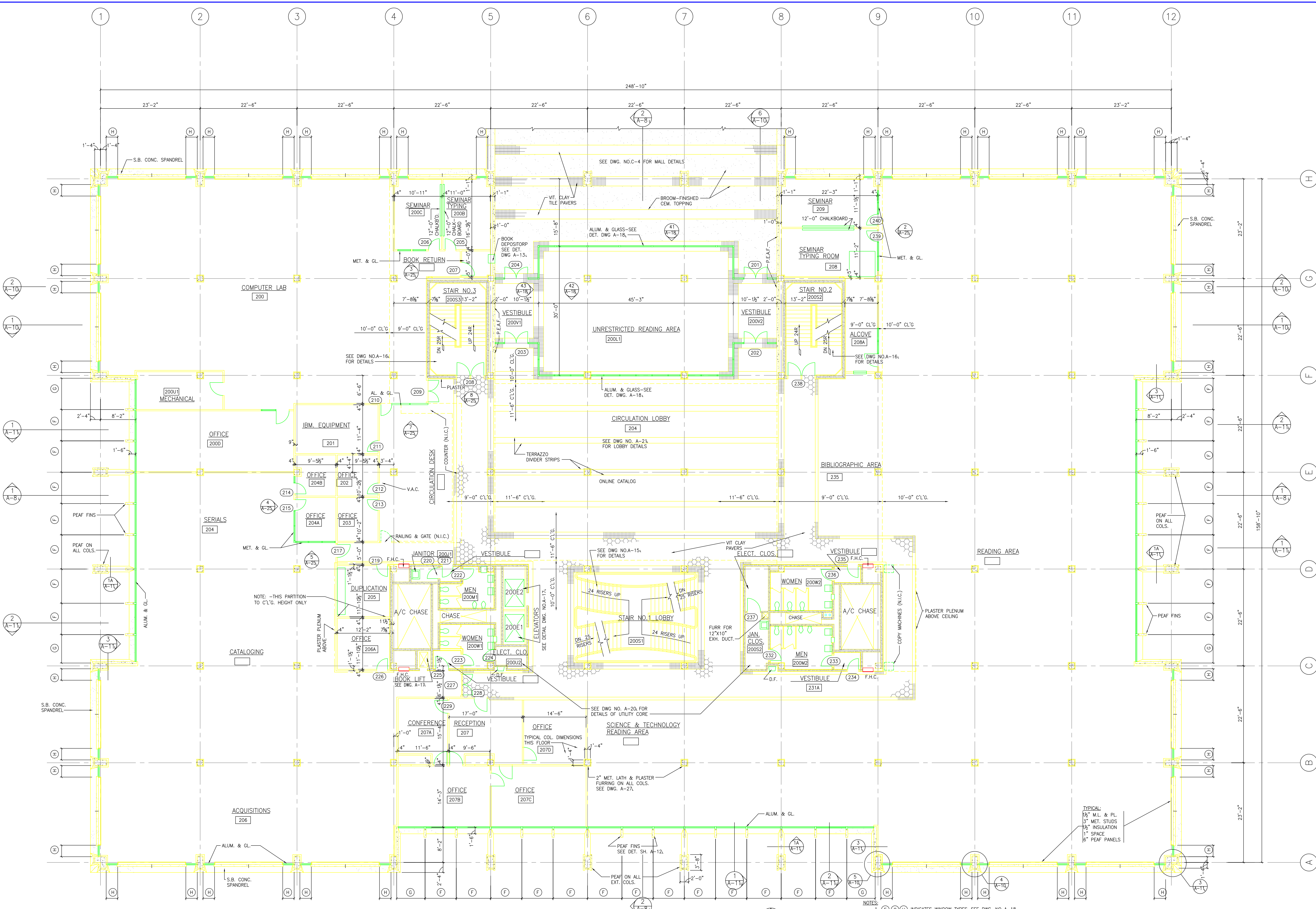
SECOND FLOOR PLAN SCALE: 1/8" = 1'-0"
