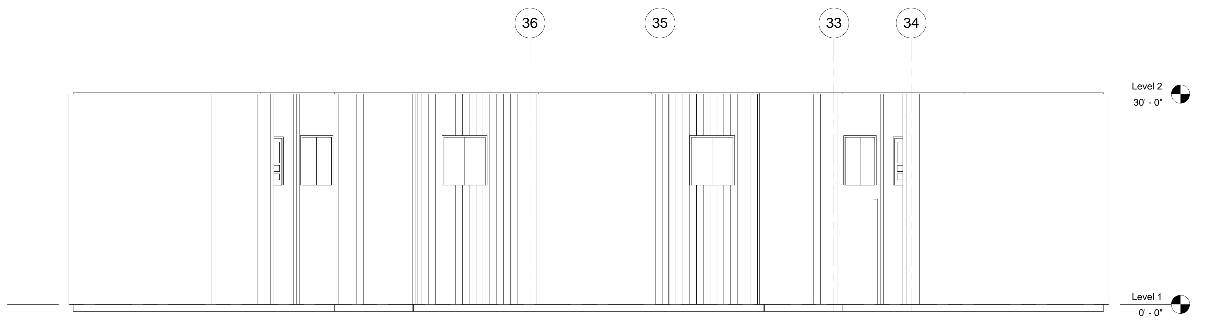
4 west elevation 1 : 100
