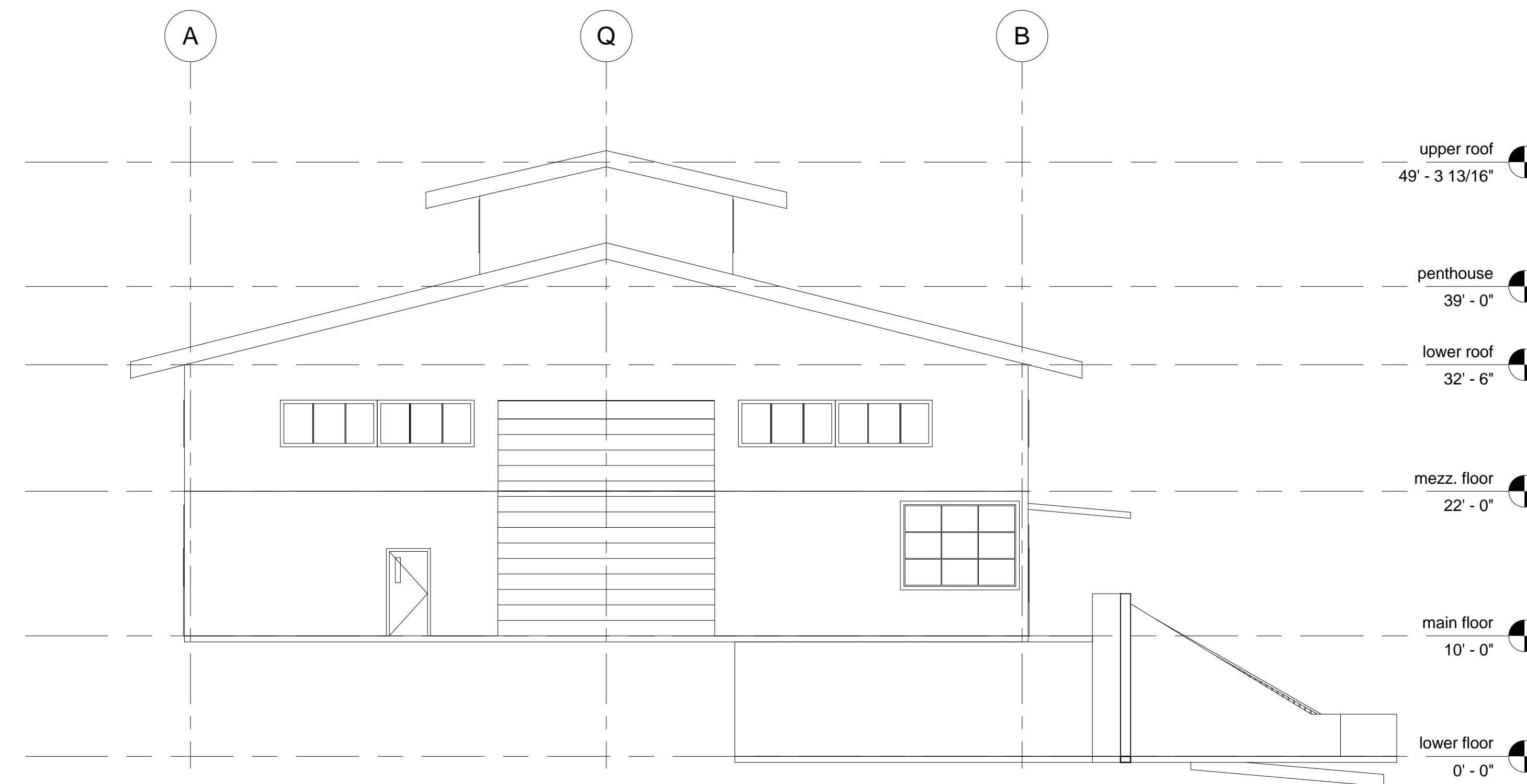
4 West 1:100
