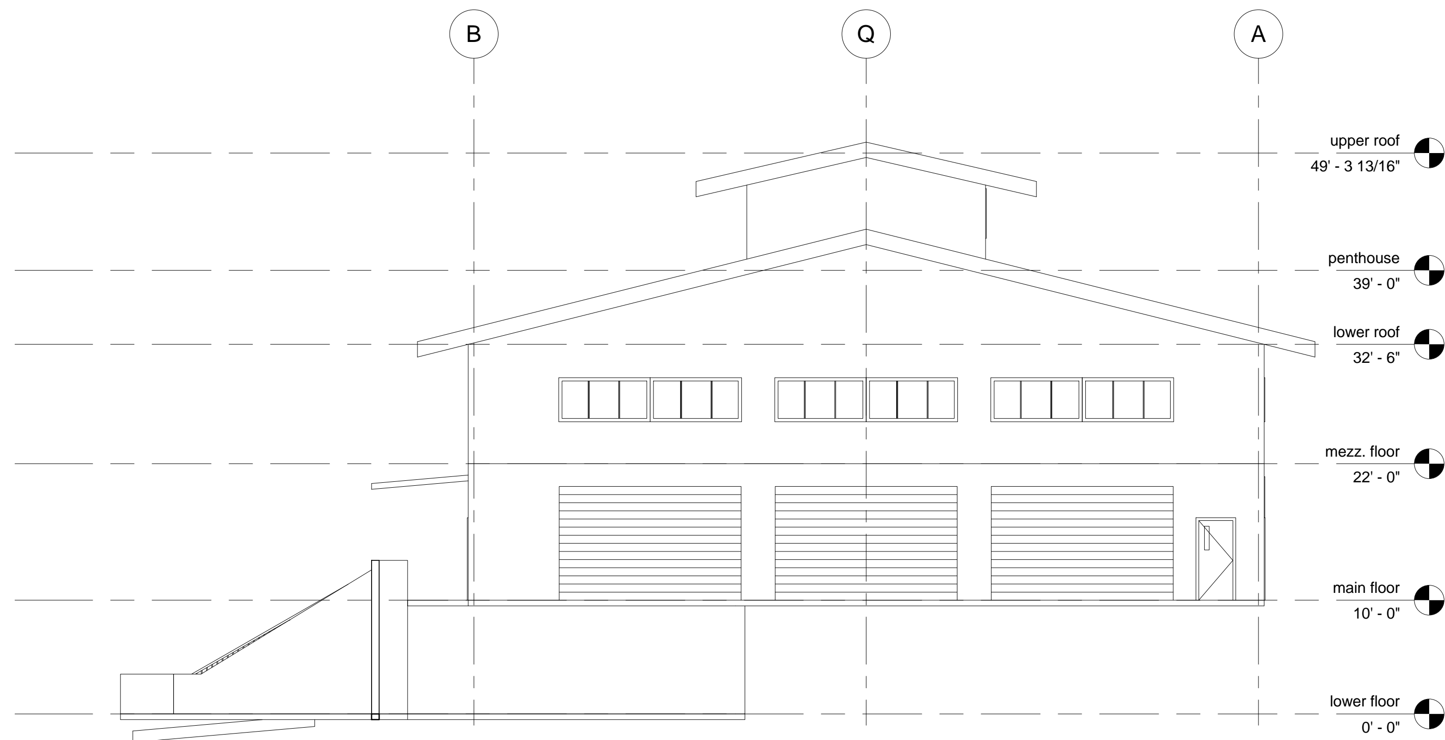
1 East 1:100
