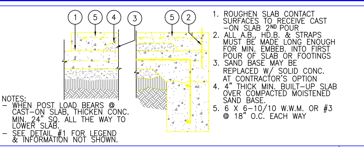
BUILT-UP SLAB 13
