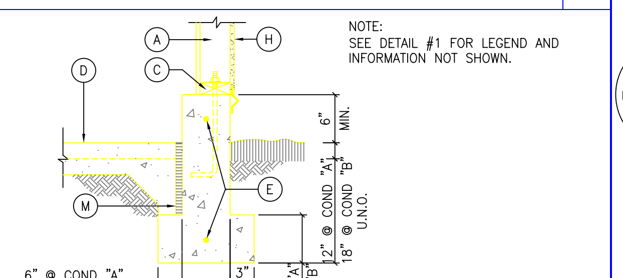
EXT. BEARING GARAGE CURB 3
