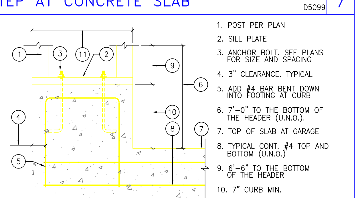
RAISED CURB 8
