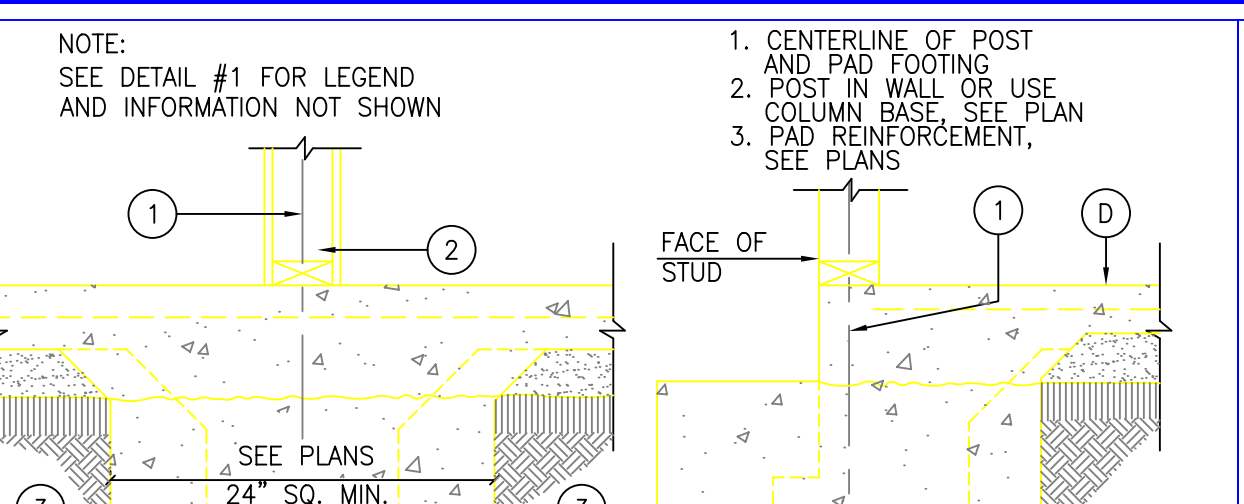
ISOLATED PAD FOOTING 6
