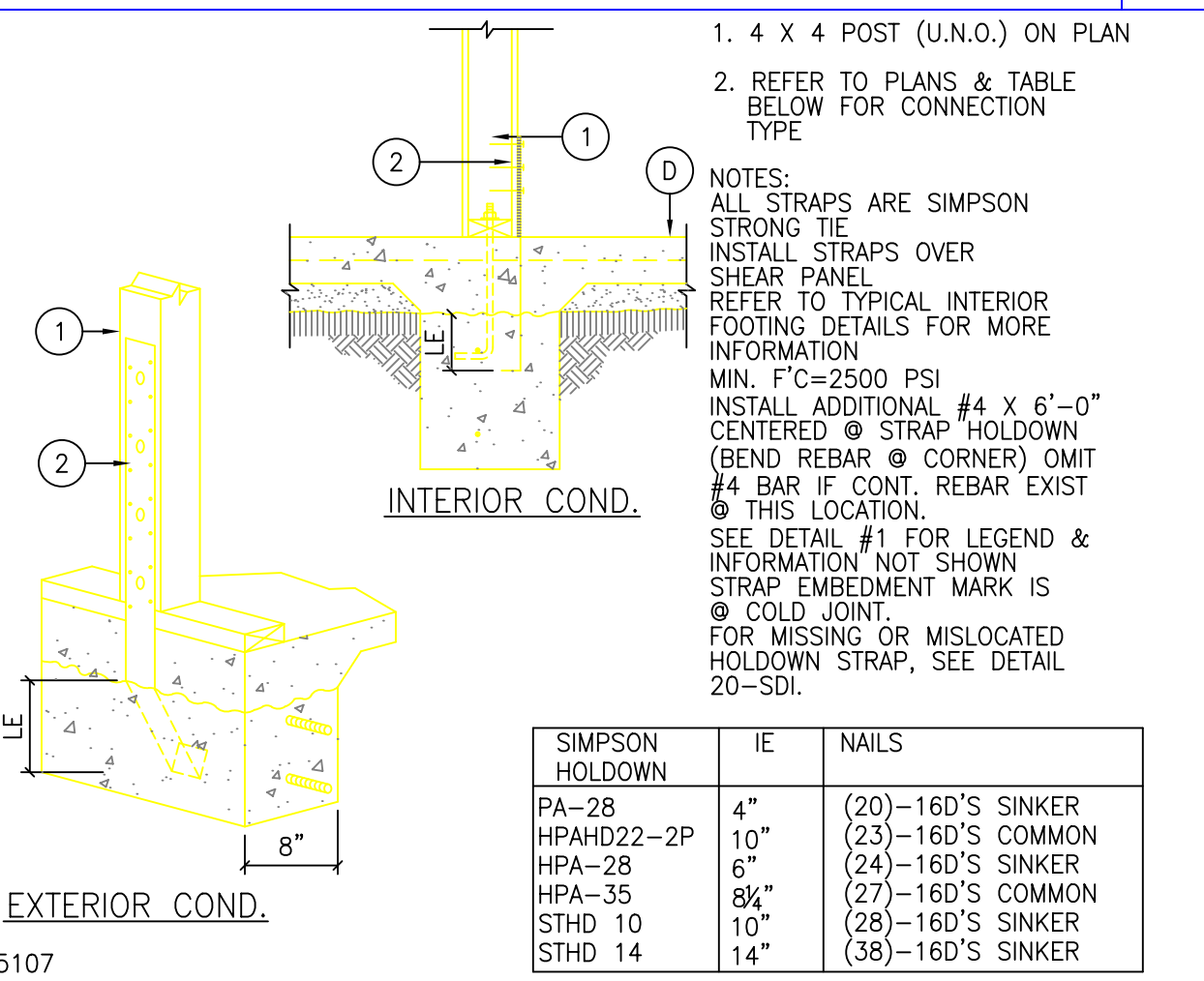
HOLDOWN STRAP 16
