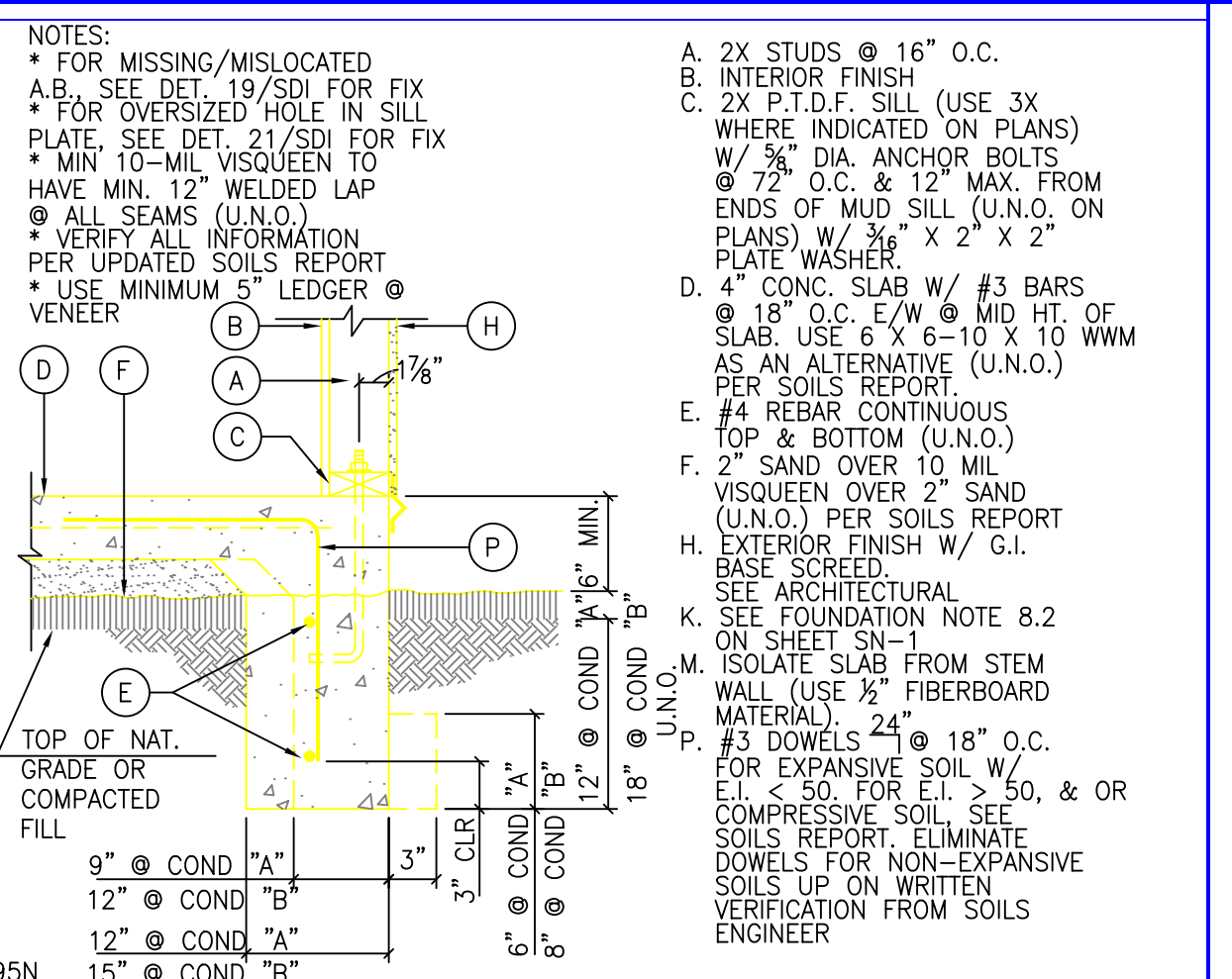
TYPICAL EXTERIOR FOOTING 1
