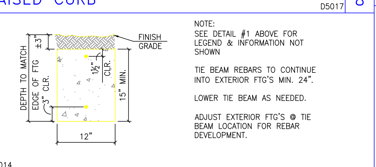
TIE BEAM 9
