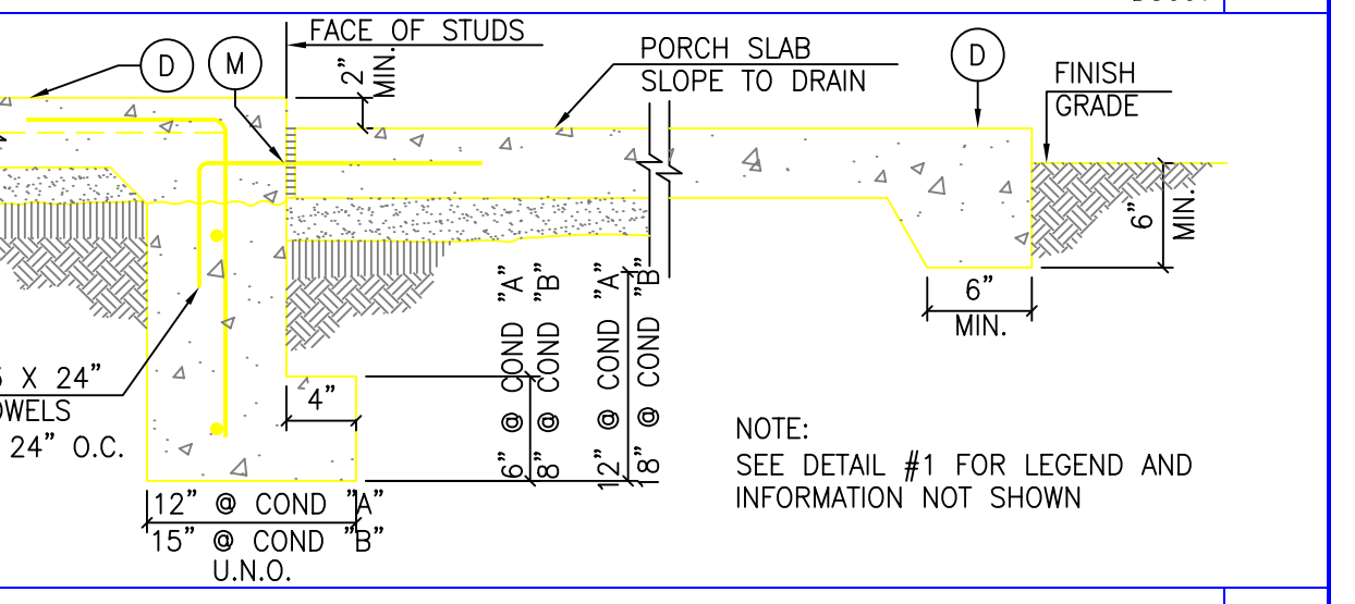
HOUSE TO PORCH 5
