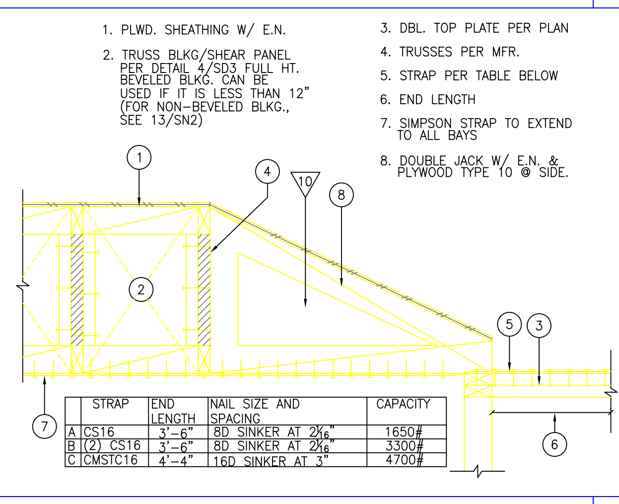
FIX FOR MISSING HOLDOWN 20
