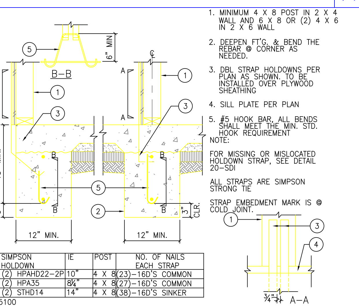
HOLDOWN STRAP 15
