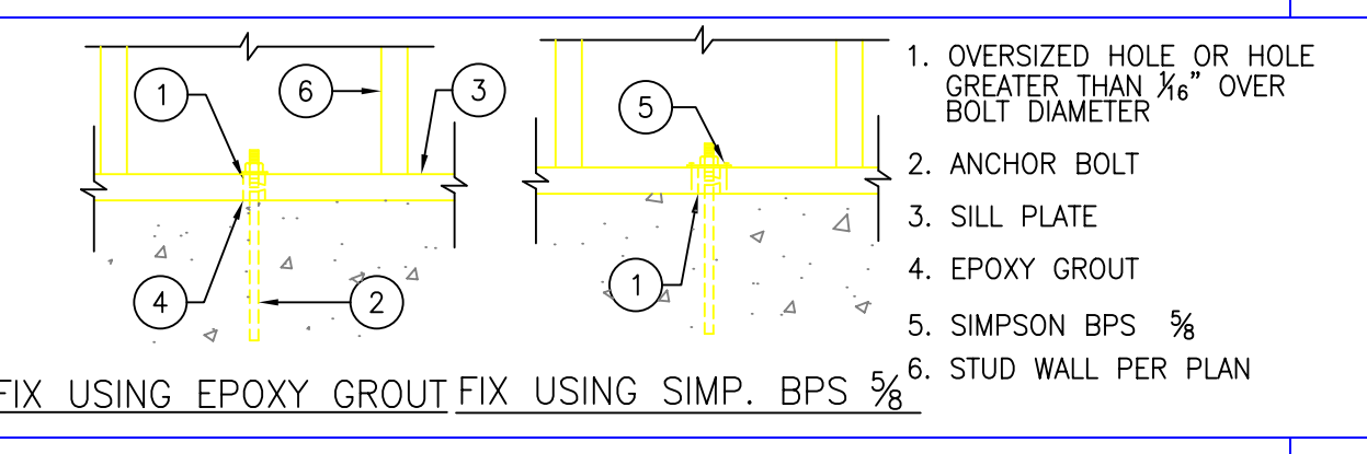
FIX FOR OVERSIZED HOLE 21
