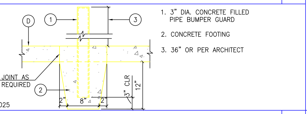
PIPE COLUMN 12
