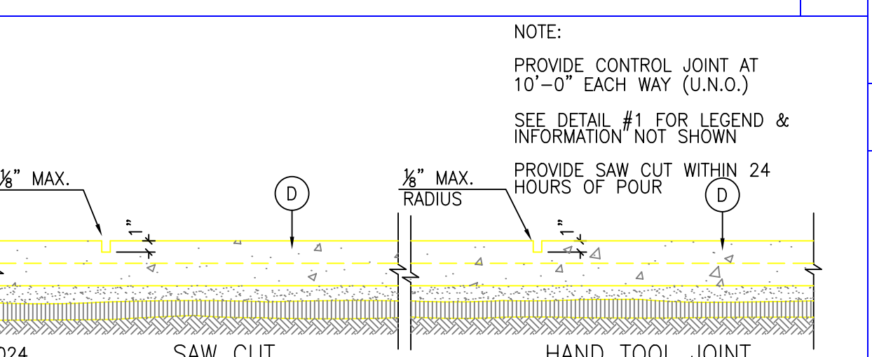
TYP. CONTROL JOINT 10
