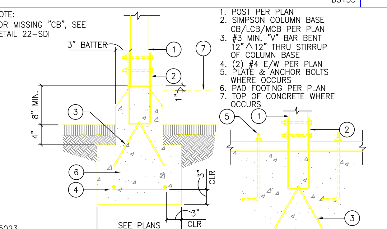
COLUMN BASE 14
