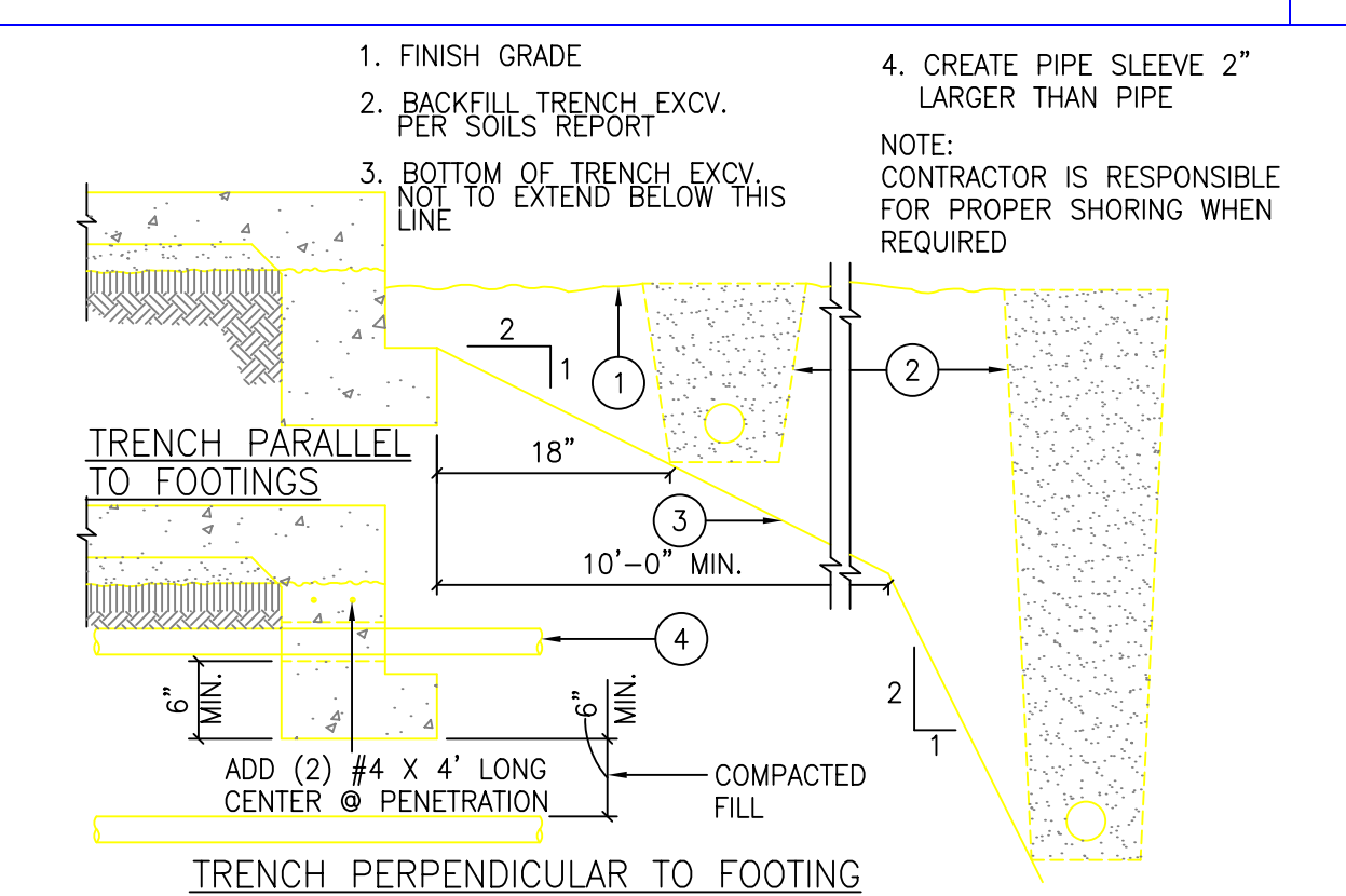
TYP. TRENCH @ FOOTINGS 24
