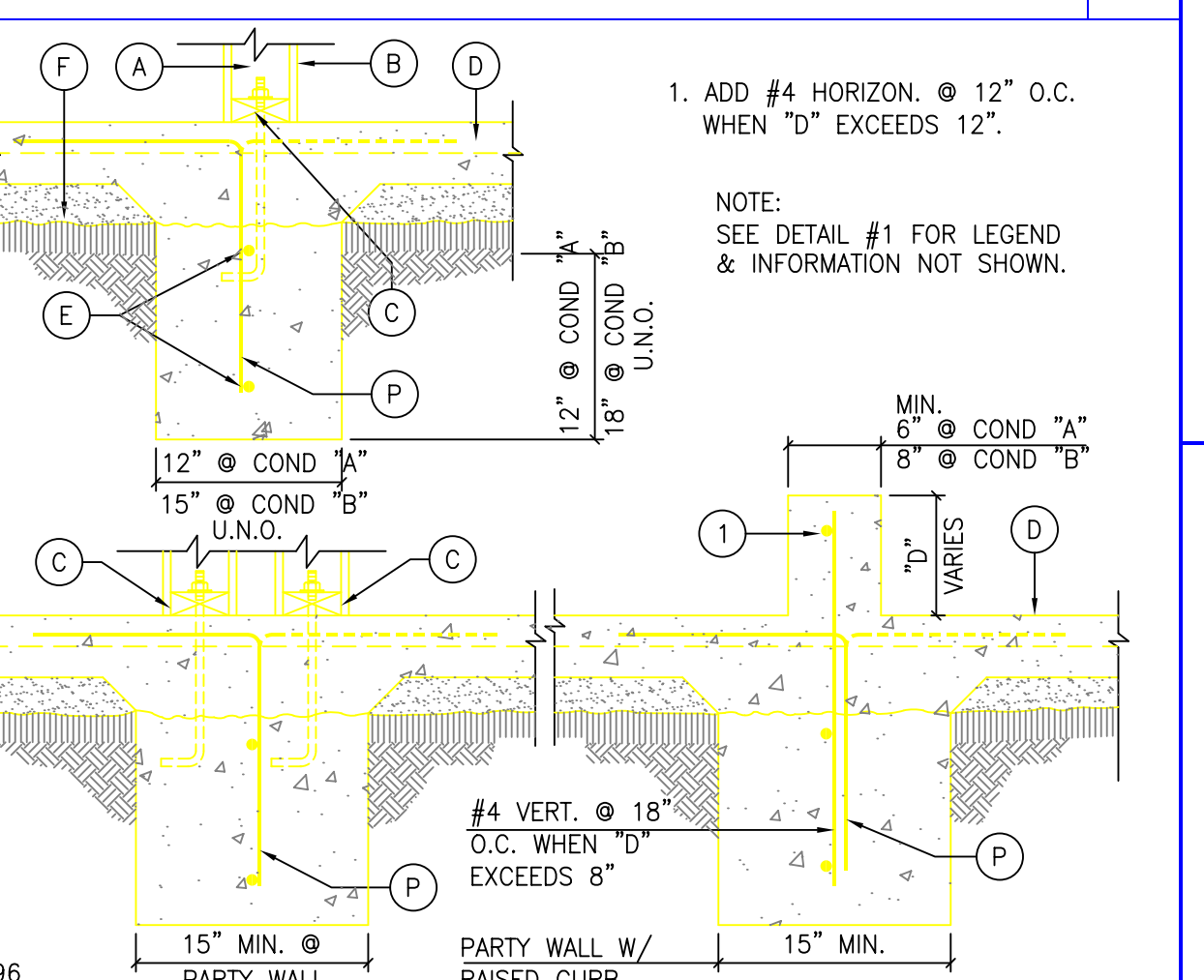
INTERIOR BEARING FOOTING 2
