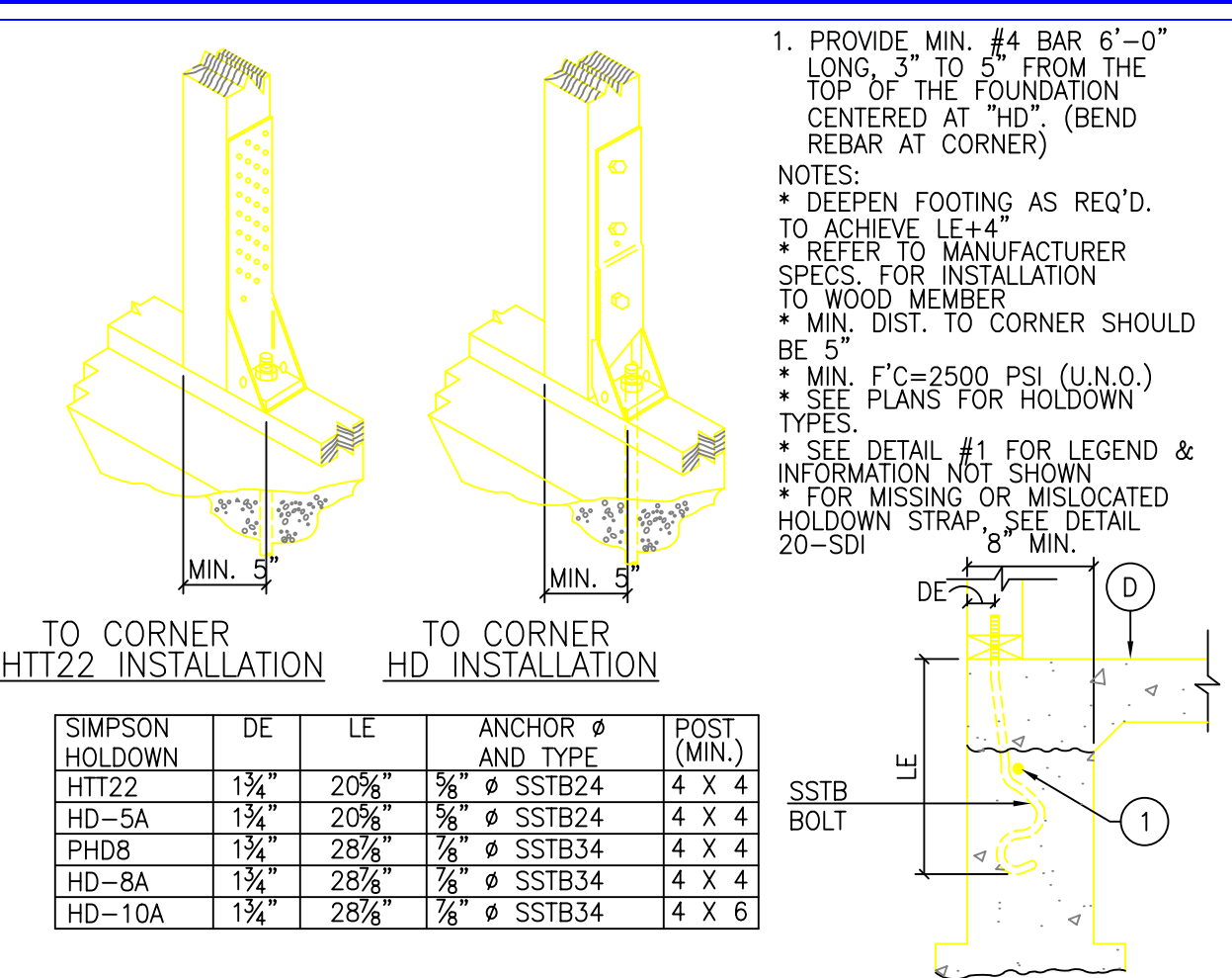
TYP. HOLDOWN INSTALLATION 18
